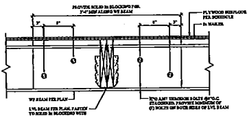
2 TYP. LVL BEAM TO WF BEAM CONN SCALE: 1-1/2" = 1'-0"
