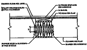
3 TYP. JOIST TO WF BEAM CONN SCALE: 1-1/2" = 1'-0"
