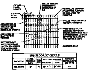
1 TYP. FLOOR SUBFLOOR ATTACHMENT SCALE: 1-1/2" = 1'-0" N.T.S.
